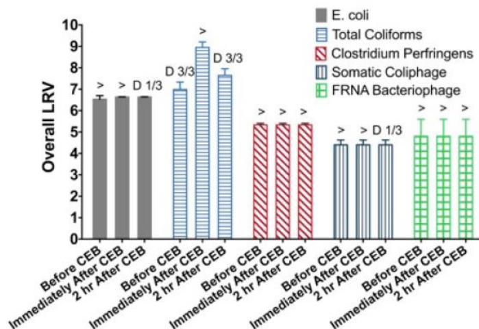
Figure 9. LRV before and after CEB with NaOCl. '>' indicates permeate concentrations below LOD. Fractions indicate the number of permeate trials at or above LOD
