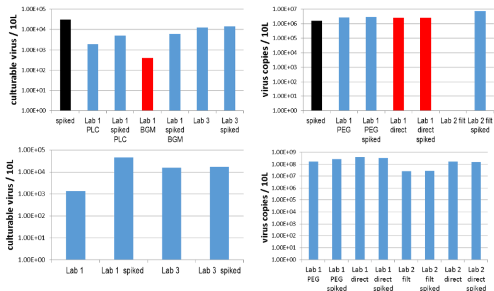
Figure 7. Virus comparison data in primary effluent, for enterovirus by culture (top left panel) and PCR (top right panel) and for adenovirus by culture (bottom left panel) and PCR (bottom right panel).
